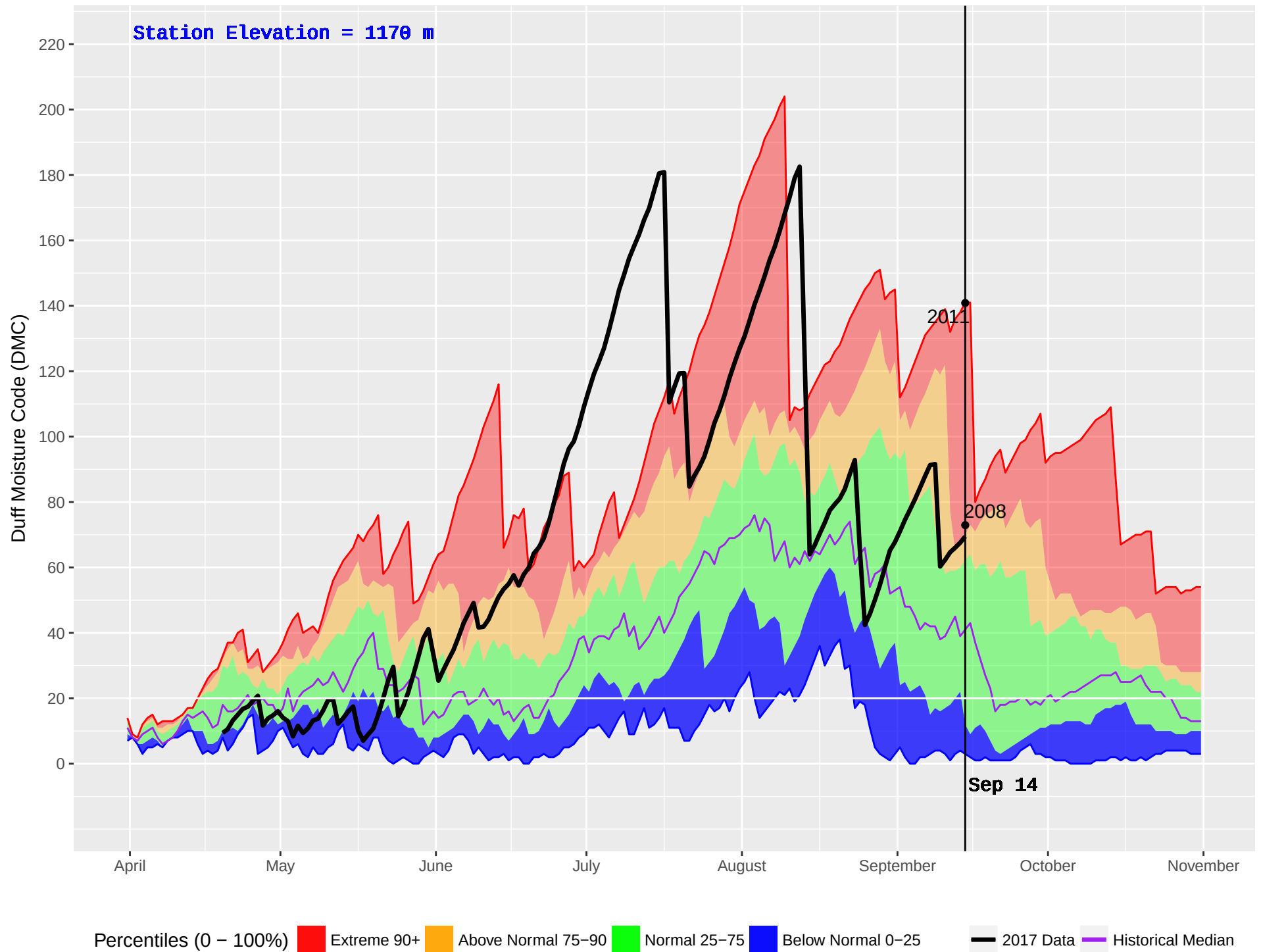
YOUNG LAKE (235) : Historical (2001–2016) and Current (2017) Noon Duff Moisture Code (DMC)
